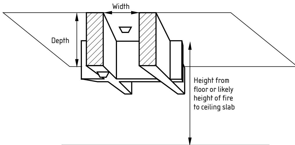
Figure 10b) — Horizontal ceiling comprising a series of small cells [see 22.3k]
